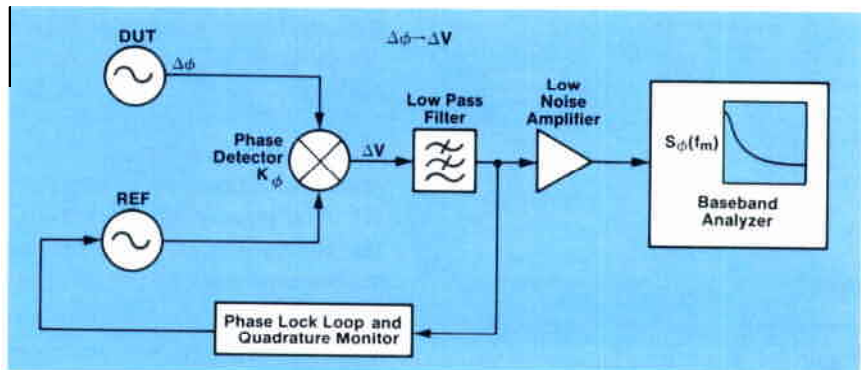
Figure 3.3. Basic phase detector method.
