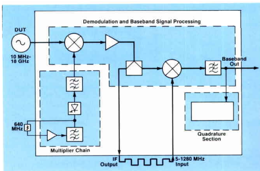
Figure 4.1. HP 11729C simplified block diagram.
