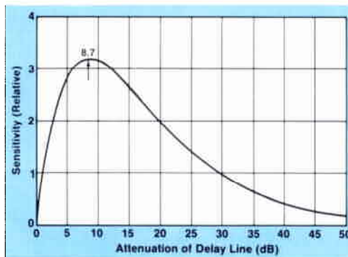
Figure C.1. System sensitivity vs. delay line attenuation.
