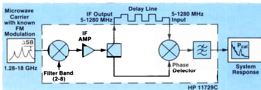
Figure 5.4. Calibrating the HP 11729C delay line/mixer frequency discriminator with a microwave source.
