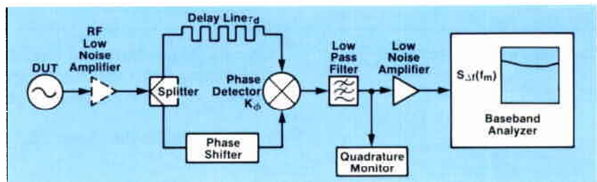
Figure 3.6. Delay line/mixer frequency discriminator.
